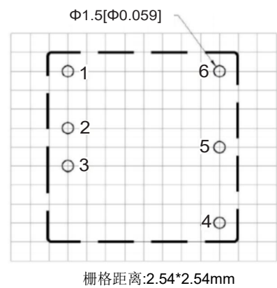
栅格距离:2.54*2.54mm
