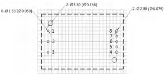
栅格距离:2.54*2.54mm
