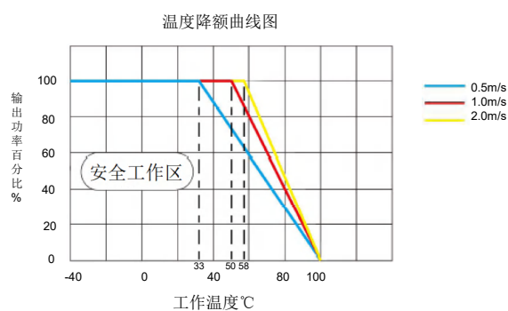
CFED100-48S28F(Vin=48V DC )
