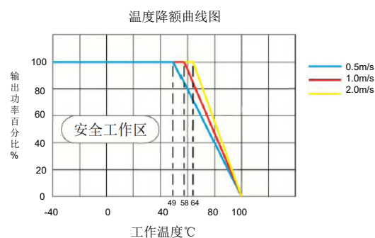
CFED100-48S24F(Vin=48V DC )
