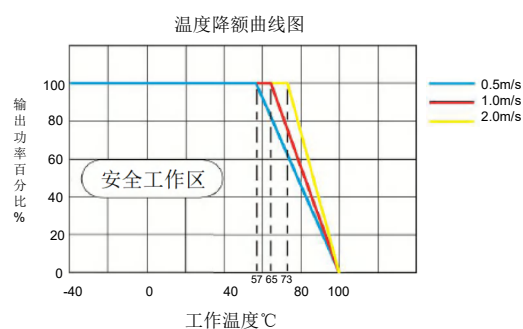
CFED100-48S05F(Vin=48V DC )
