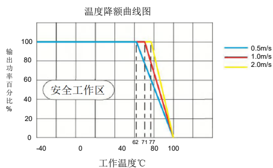
CFED100-48S15F(Vin=48V DC )
