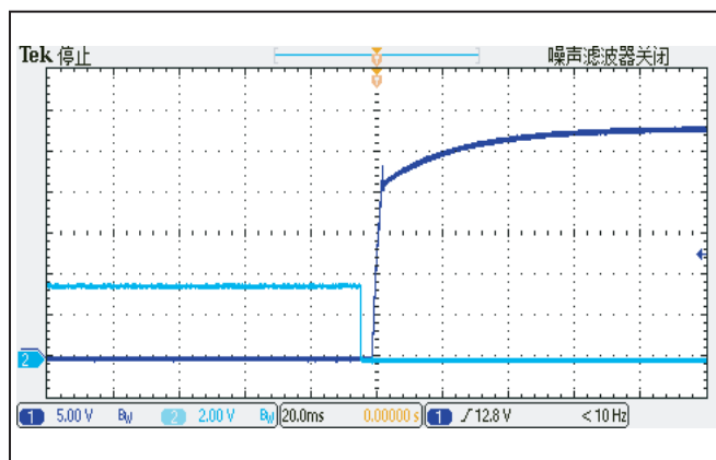
图 6: ON/OFF 启机延时, Vin=280VDC, Io=33.4A CH1: 输出电压, CH2: ON/OFF 电压, TC=25°C
