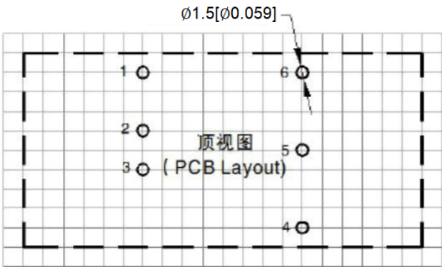
栅格距离2.54*2.54mm
