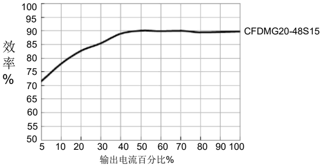
效率/输出负载(Vin=48V DC )
